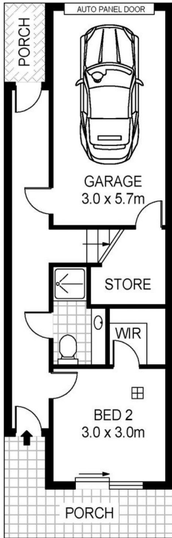
GROUND LEVEL
