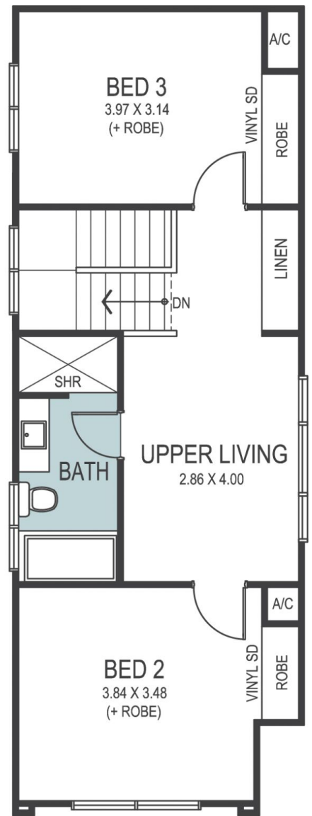
UPPER FLOOR
