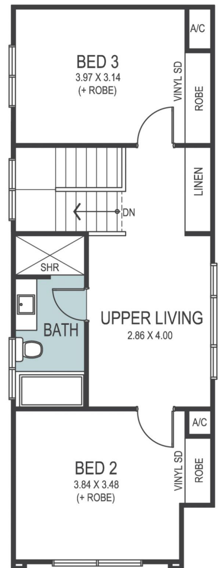
UPPER FLOOR
