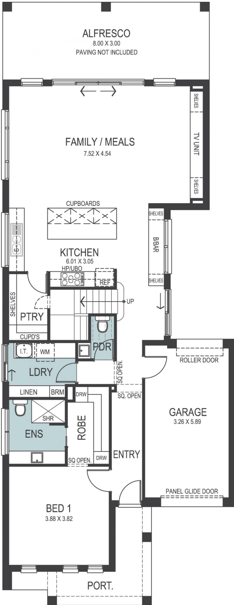
GROUND FLOOR
