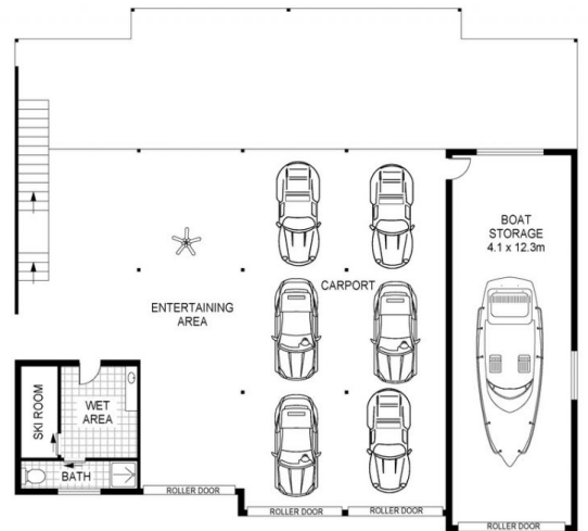
LOWER FLOOR
